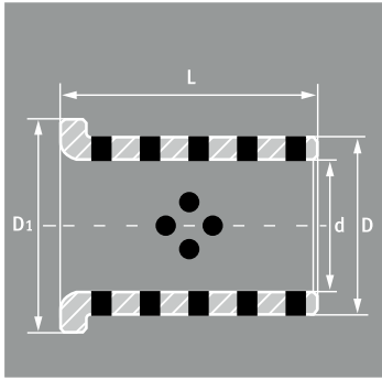
AKLF Flanged bushing
