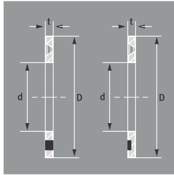
AKLW Thrust washer
