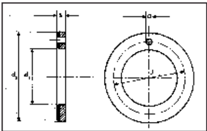
Thrust washer
